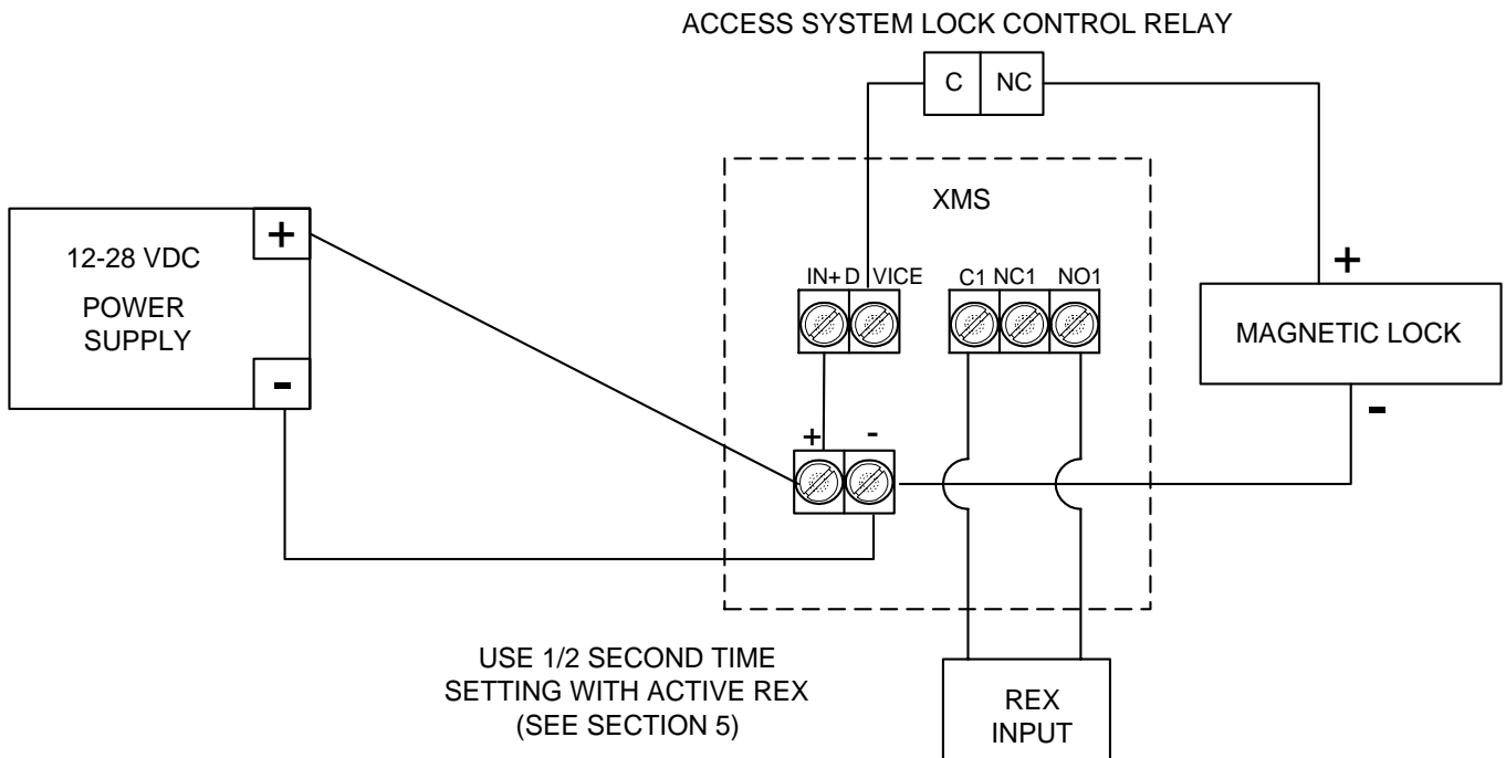
FIG. 6: WIRING WITH “GENERIC” PUSH BUTTON AND TIMER
